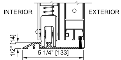
FLAT EXTRUSION UNDER "SO" PANEL ONLY
