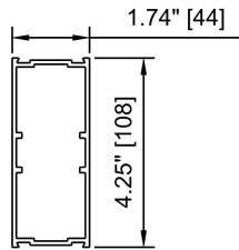
MUNTIN BAR, 4" 6063-T6
